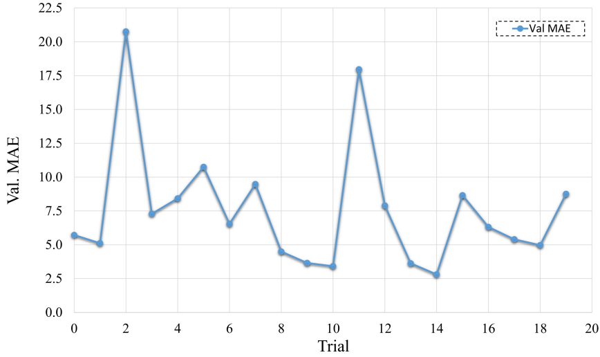
Figure 7: Validation MAE across Bayesian optimisation trials.
