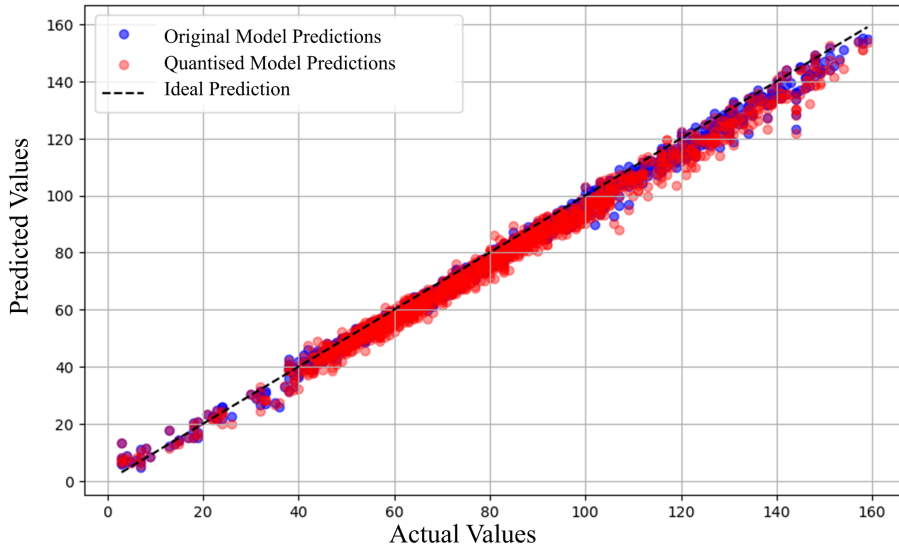
Figure 12: Comparison of quantised vs. original model predictions.
