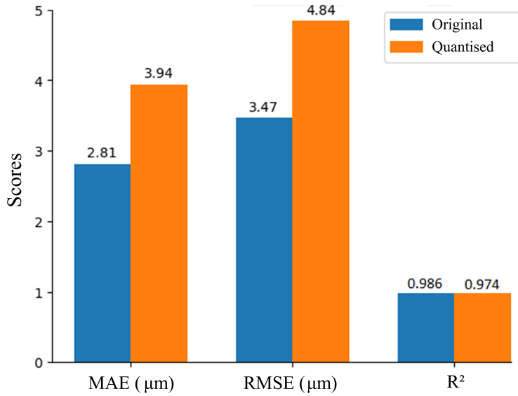
Figure 11: Comparison of scores for original and quantised models.
