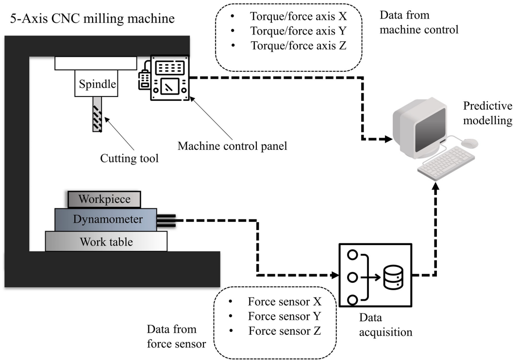
Figure 4: Process flow diagram illustrating data acquisition and predictive modelling workflow.
