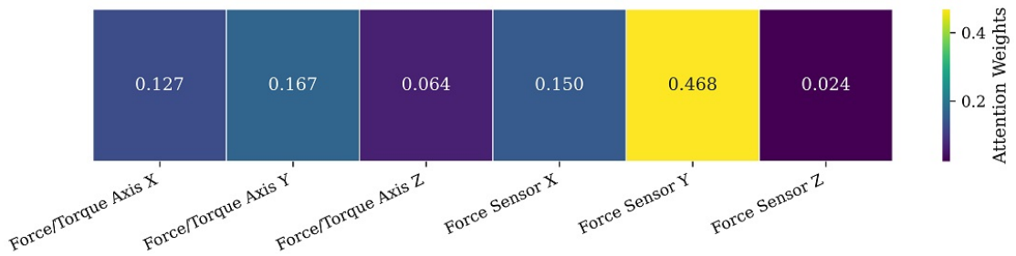
Figure 9: Attention weight distribution across sensor channels, representing the relative importance learned by the model.
