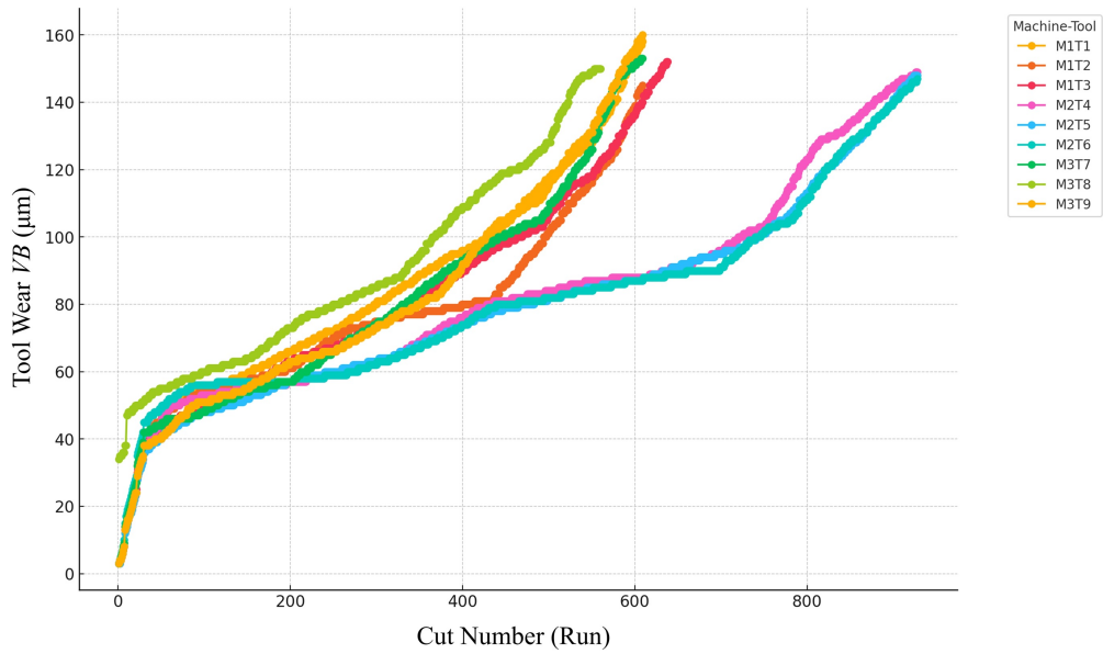
Figure 6: Tool wear progression across different tools over multiple cuts.
