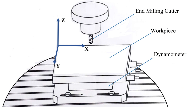
Figure 3: Schematic illustration of the experimental setup reported in [50].
