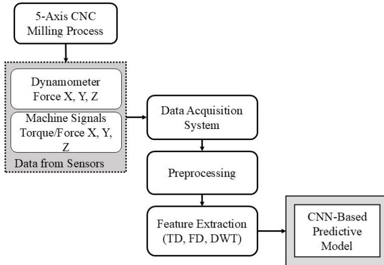
Figure 5: Data measurement and preprocessing chain diagram illustrating data acquisition and predictive modelling workflow.
