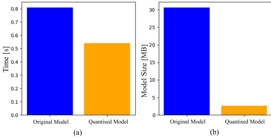
Figure 10: Comparison of models' inference time (a) and size (b).
