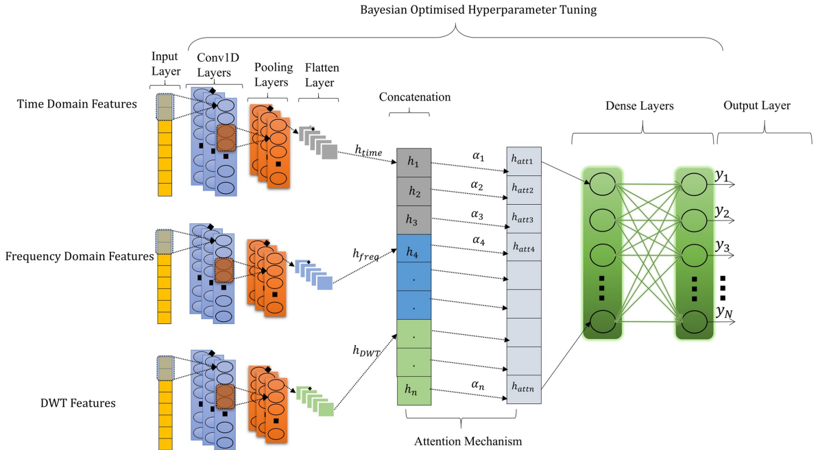
Figure 2: Multi-CNN with attention mechanism and Bayesian optimisation for hyperparameters tuning.
