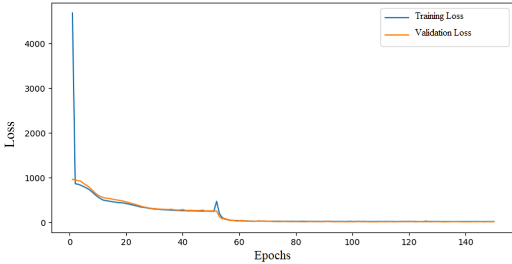
Figure 8: Training and validation loss curve.
