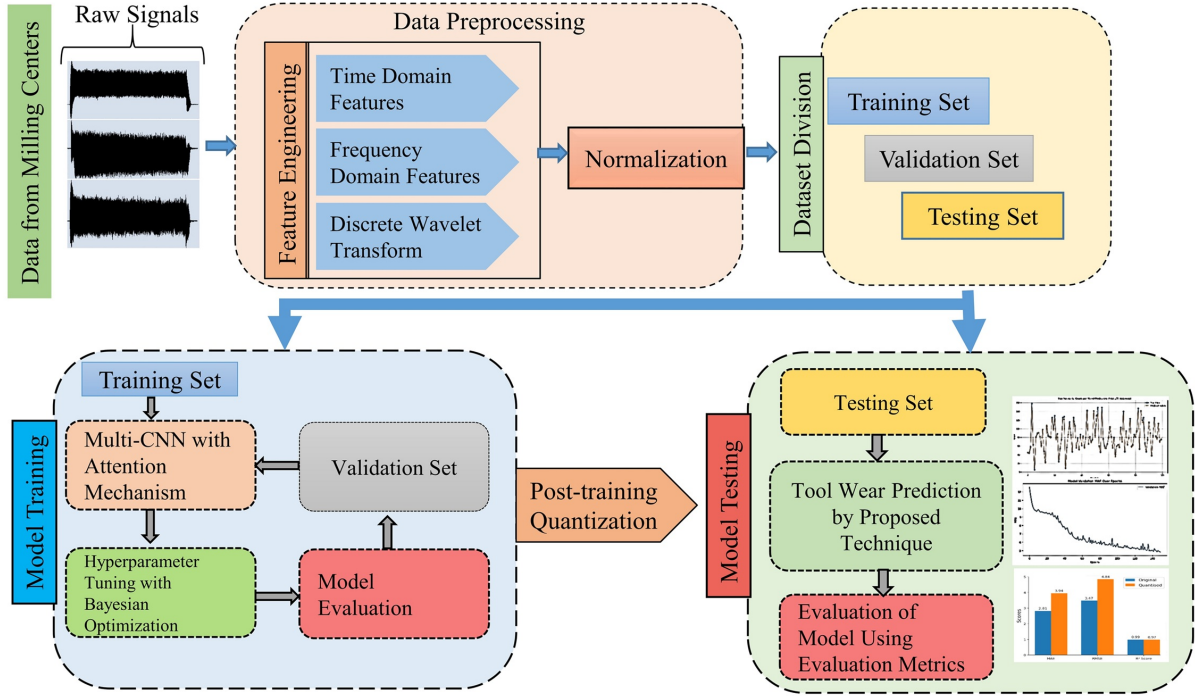
Figure 1: Flow diagram illustrating the proposed Multi-CNN-based approach for tool wear prediction.
